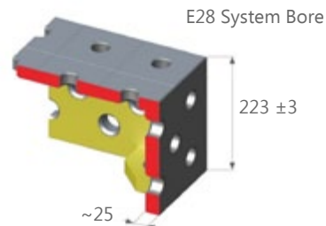
Dimensional data
